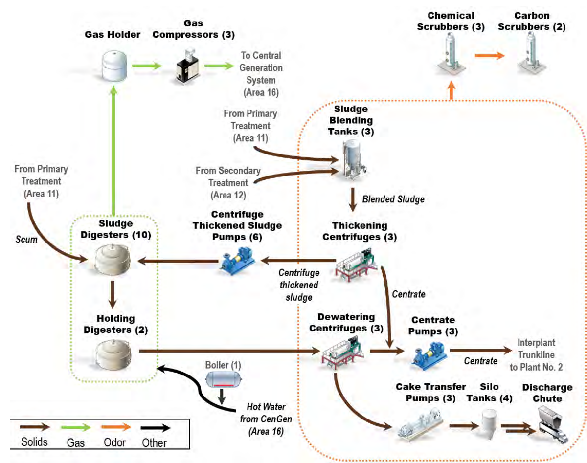
Process Schematic
