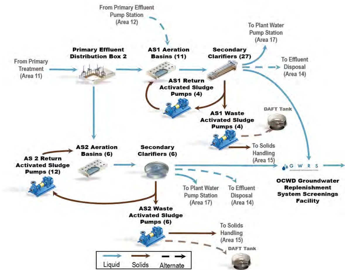
Process Schematic
