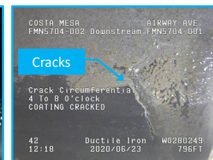
Gravity Sewer
