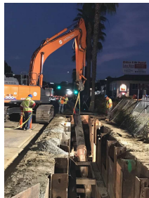
Pipe upsizing via pipe bursting
