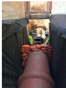
Pipe replacement via open cut
