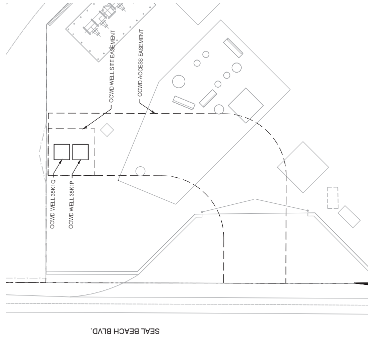
OCWD WELLS PLAN SCALE: 1" = 10'
