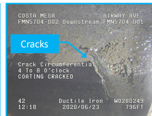
Gravity Sewer
